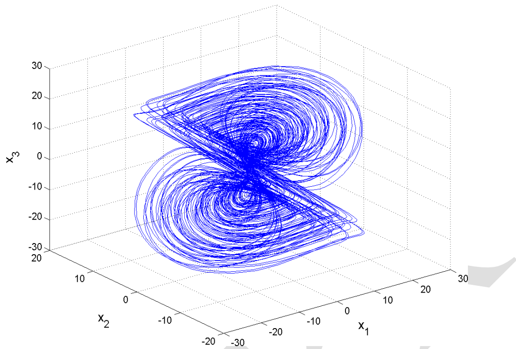
Figure 3. Chaotic Portrait of the Liu Four-Wing Attractor
