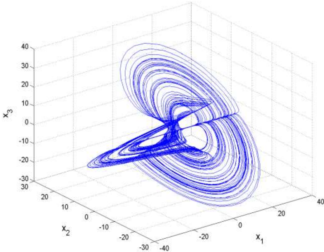
Figure 1. Chaotic Portrait of the Liu-Chen Four-Scroll Attractor
