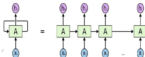
Fig. 2: A simple neural network unrolled into simple neural network.
