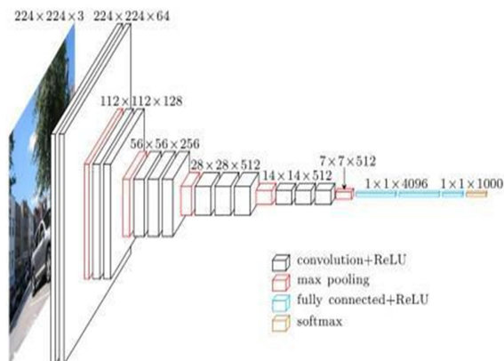
Fig.1: CNN Architecture
