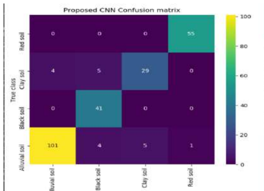
Fig. Confusion matrix for soil classification and plant recommendation
