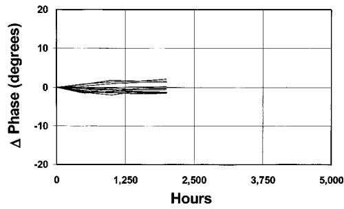
Fig. 12. Phase drift for 2.5 Gb/s bias free, x-cut, APE modulators at (a) 85 and (b) 100 C [19].
