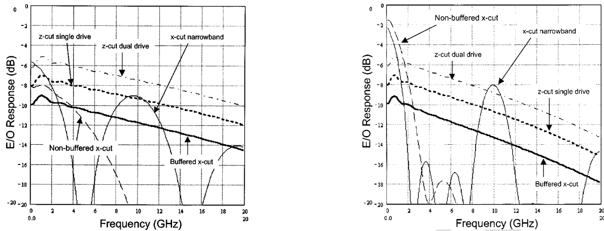
Fig. 4. Calculated electrooptic response for several devices designed for broad-band digital or RZ pulsing applications at 2.5 or 10 Gb/s using conventional electrode and waveguide structures (no ridges or \epsilon_n enhancement). Electrode lengths were chosen to be representative of devices used in actual applications and are shown in Table I.
