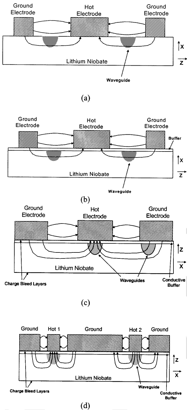
Fig. 3. Most common electrode configurations for (a) nonbuffered x-cut, (b) buffered x-cut, (c) buffered single-drive z-cut, and (d) buffered dual drive z-cut.
