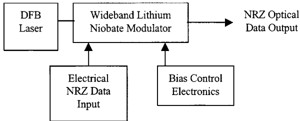
Fig. 6. Data modulator topology for NRZ transmission.
